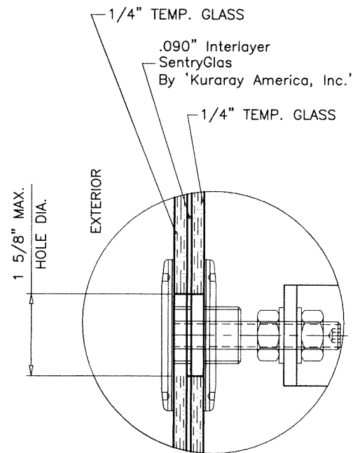
GLASS TYPE 'A' 9/16" OVERALL NOMINAL THK.
