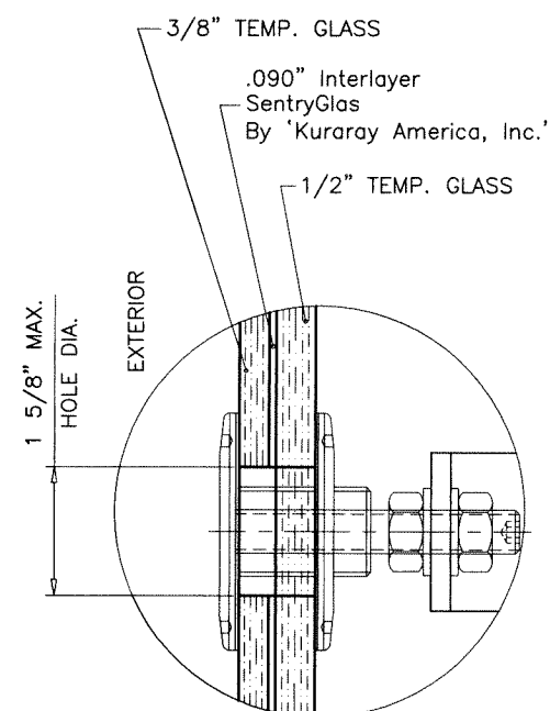
GLASS TYPE 'C' 15/16" OVERALL NOMINAL THK.
