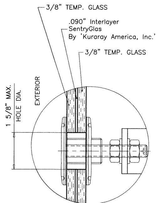
GLASS TYPE 'B' 13/16" OVERALL NOMINAL THK.
